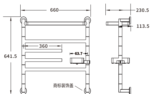
K-35634T/K-35634T-S/K-35634T-L(带储物盒)
